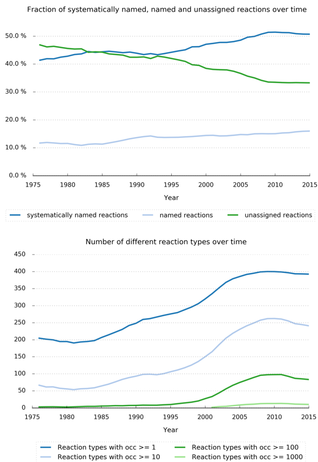
Figure 2. Top: Evolution of classified and unclassified unique reactions over time. Classified reactions are further subdivided in reactions with systematic names and named reactions. Bottom: Evolution of the number of different reaction types showing up in all patents per year. Note that the values in both plots were smoothed/averaged over 5 years for better visual clarity.
