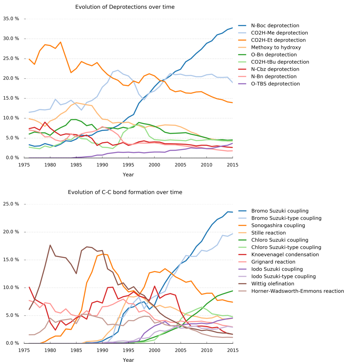
Figure 6. Top: Evolution of third largest reaction class deprotections over time. Bottom: Evolution of fourth largest reaction class C–C bond formations over time. Note that in Suzuki-type couplings , since the palladium catalyst could not always be correctly text-mined from the patent, these subtypes have been introduced. In both plots reaction types that represent at least 2% of the data were shown. Note that the values in both plots were smoothed/averaged over 5 years for better visual clarity.
