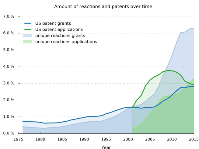
Figure 1. Distribution of U.S. patents and unique reactions extracted from those per year in the time period comprising the years from 1976 until October 2015. Only patents with ICP code A61K 21 (excluding A61K/8) were considered. In light blue and blue, unique reactions of granted U.S. patents and granted U.S. patents are shown, respectively. In light green and green, unique reactions of U.S. patent applications and U.S. patent applications are shown, respectively. Applications only date back to 2001. Note that the values in the plot were smoothed/averaged over 5 years for better visual clarity.
