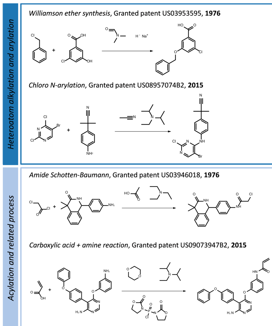
Figure 4. Exemplary reactions for the two largest reaction classes heteroatom alkylation and arylation and acylation and related processes . For each class the most frequently used reaction types for the years 1976 and 2015 are shown.
