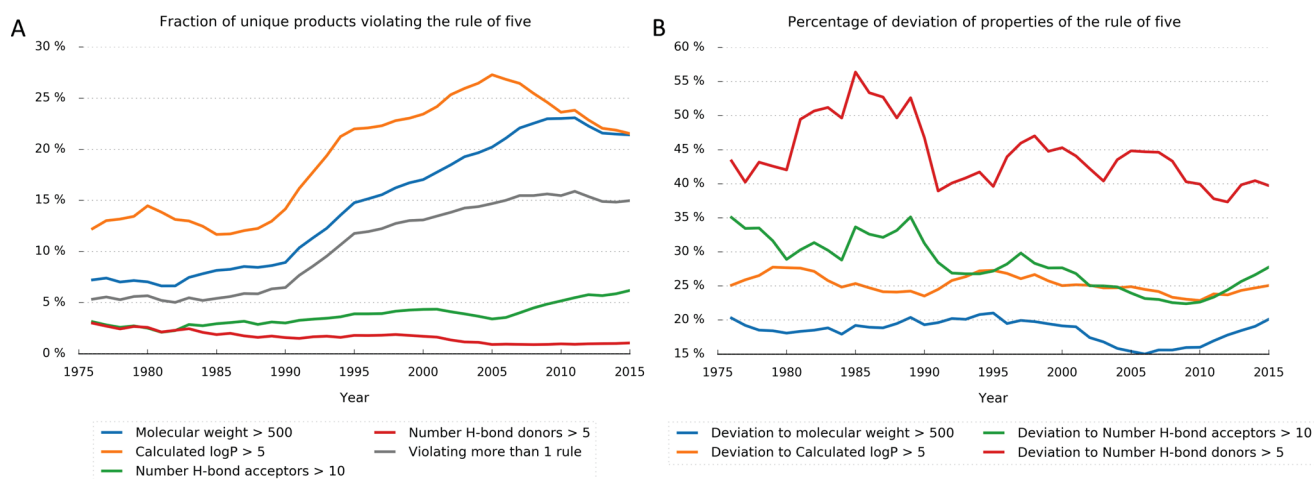
Figure 13. (A) Fraction of reaction products violating Lipinski's rule of five over time. Products that violate more than one rule were counted each time. (B) Percentage of deviation of the four different rule-of-five properties from their thresholds over time. In these plots a time period between the year 1976 and the year 2015 (October) was considered. Note that the values in the plots were smoothed/averaged over 5 years for better visual clarity.
