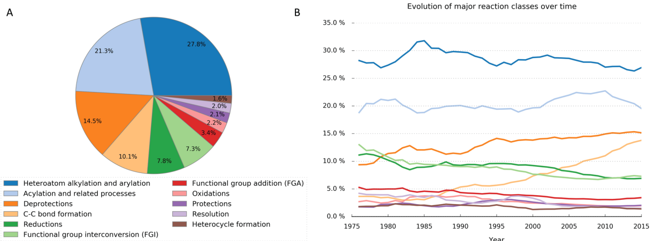
Figure 3. (A) Overall distribution of the major reaction classes of the patent reaction data set. (B) Evolution of the major reaction classes over time. Note that the values were smoothed/averaged over 5 years for better visual clarity.
