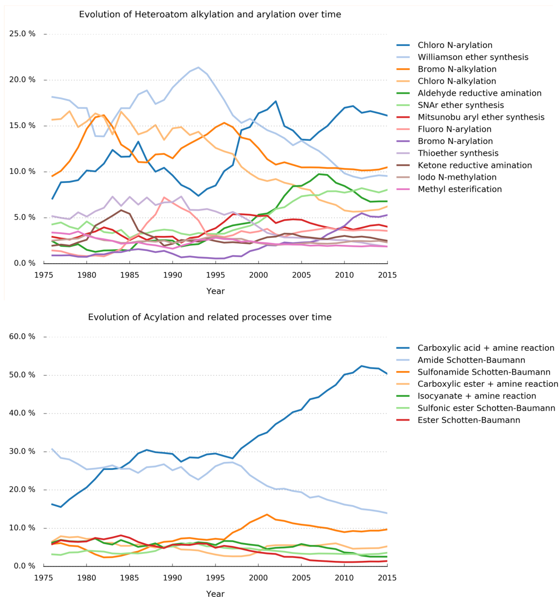
Figure 5. Top: Evolution of largest reaction class heteroatom alkylations and arylations over time. Bottom: Evolution of second largest reaction class acylation and related processes over time. In both plots reaction types that represent at least 2% of the data were shown. Note that the values in both plots were smoothed/averaged over 5 years for better visual clarity.
