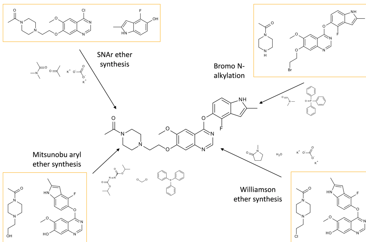
Figure 10. Exemplary product that has been made by four different reaction types. The product molecule and the four different routes stem from U.S. patent US07268230B2.
