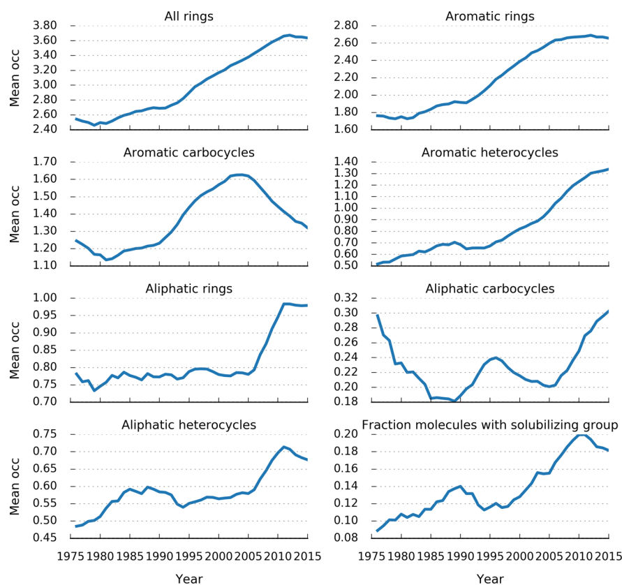
Figure 11. Evolution of the mean number of rings in reaction products over time. In these plots a time period between the year 1976 and the year 2015 (October) was considered. Note that the values in the plots were smoothed/averaged over 5 years for better visual clarity.
