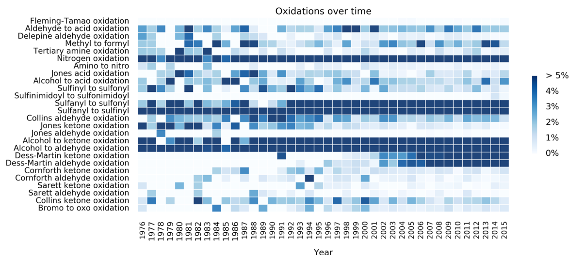
Figure 7. Evolution of oxidations over time. In the plot all reaction types found at least once over the whole time period were shown. Values were normalized by the yearly number of reactions in this reaction class.
