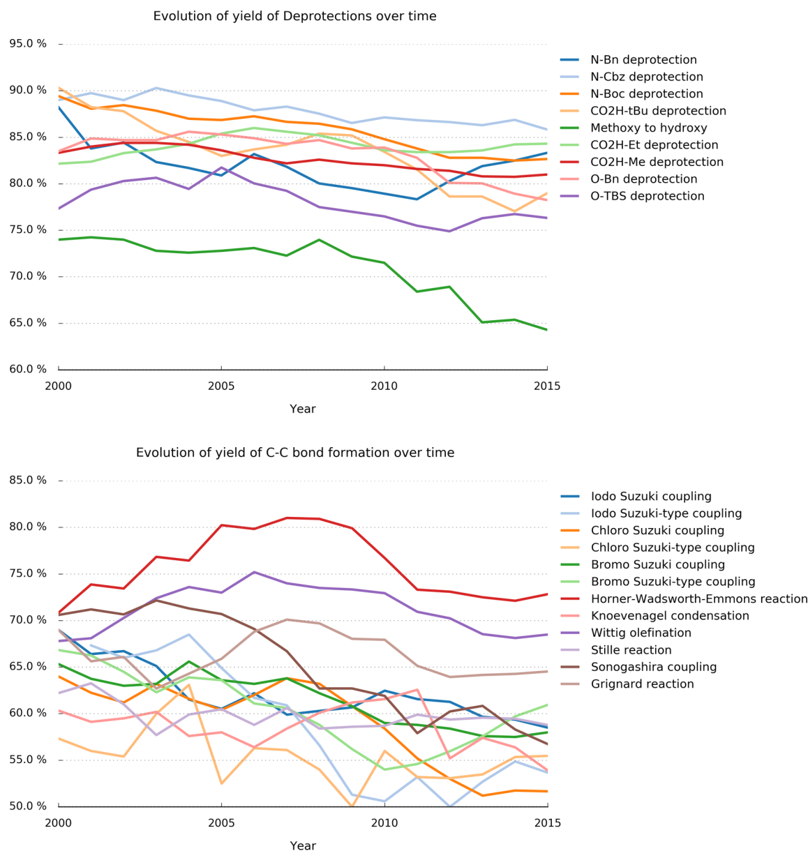
Figure 9. Top: Evolution of the median yield of deprotections over time. Bottom: Evolution of the median yield of the C–C bond formation over time. Note that in Suzuki-type couplings the palladium agent could not correctly be text-mined from the patent; due to this, these subtypes have been introduced. In these plots a time period between the year 2000 and the year 2015 (October) was considered. In both plots reaction types that represent at least 2% of the data were shown. Note that the values in both plots were smoothed/averaged over 5 years for better visual clarity.
