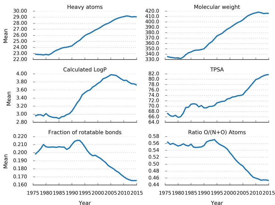
Figure 12. Evolution of the mean number of different structural and global properties of reaction products over time. The fraction of rotatable bonds was normalized by the number of bonds. In these plots a time period between the year 1976 and the year 2015 (October) was considered. Note that the values in the plots were smoothed/averaged over 5 years for better visual clarity.
