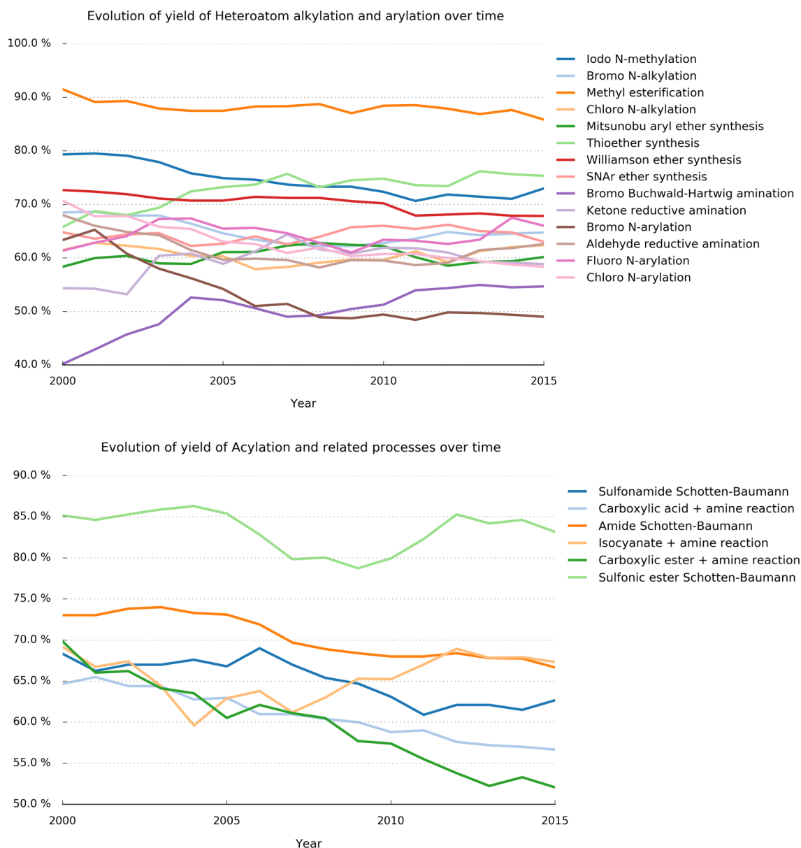
Figure 8. Top: Evolution of the median yield of heteroatom alkylations and arylations over time. Bottom: Evolution of the median yield of the acylation and related processes over time. In these plots a time period between the year 2000 and the year 2015 (October) was considered. In both plots reaction types that represent at least 2% of the data were shown. Note that the values in both plots were smoothed/averaged over 5 years for better visual clarity.
